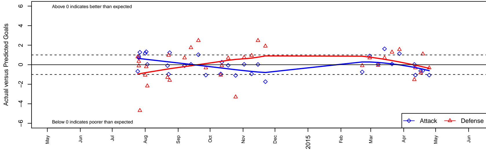
Kitsap Pumas G02 Dots are actual minus expected GF (blue circles) and GA (red triangles). Blue line is smoothed change in attack strength. Red is smoothed change in defense strength.
